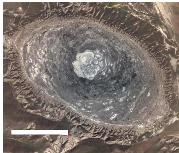
Figure 2. Mud volcano in Azerbaijan with nearly flat, pedestal-like surface and central high-albedo, sub-circular patch; 40.4° N, 49.0° E; scale bar 1 km.
