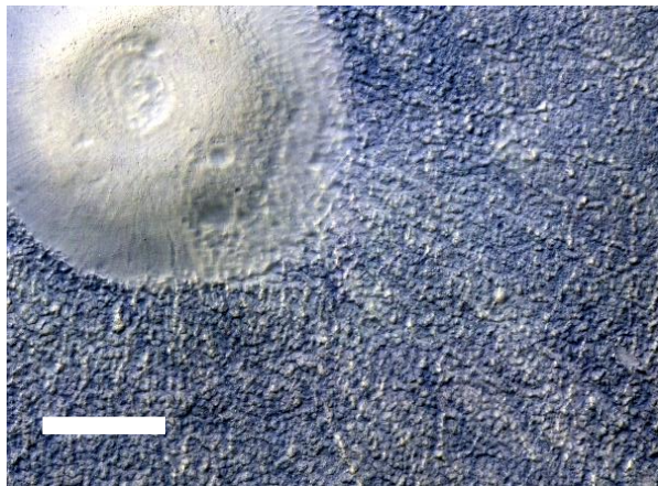
Figure 1. Mud volcano in Acidalia Planitia; HiRISE PSP_002233-2225; 42.1° N, 319.3° E; scale bar 200 m.
