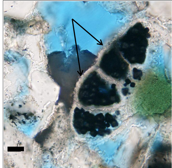
Figure 4. Optical photomicrograph (transmitted light) of rock breccia from the Bozdag mud volcano in Azerbaijan; arrows indicate calcareous microfossil partially filled with pyrite; blue epoxy preparation; scale bar 10 \mu m.
